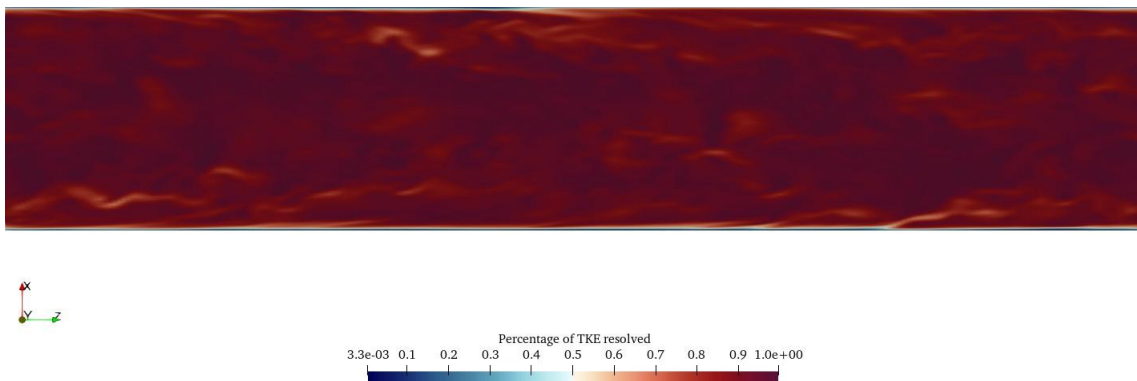
Figure 47: Fraction of resolved TKE
