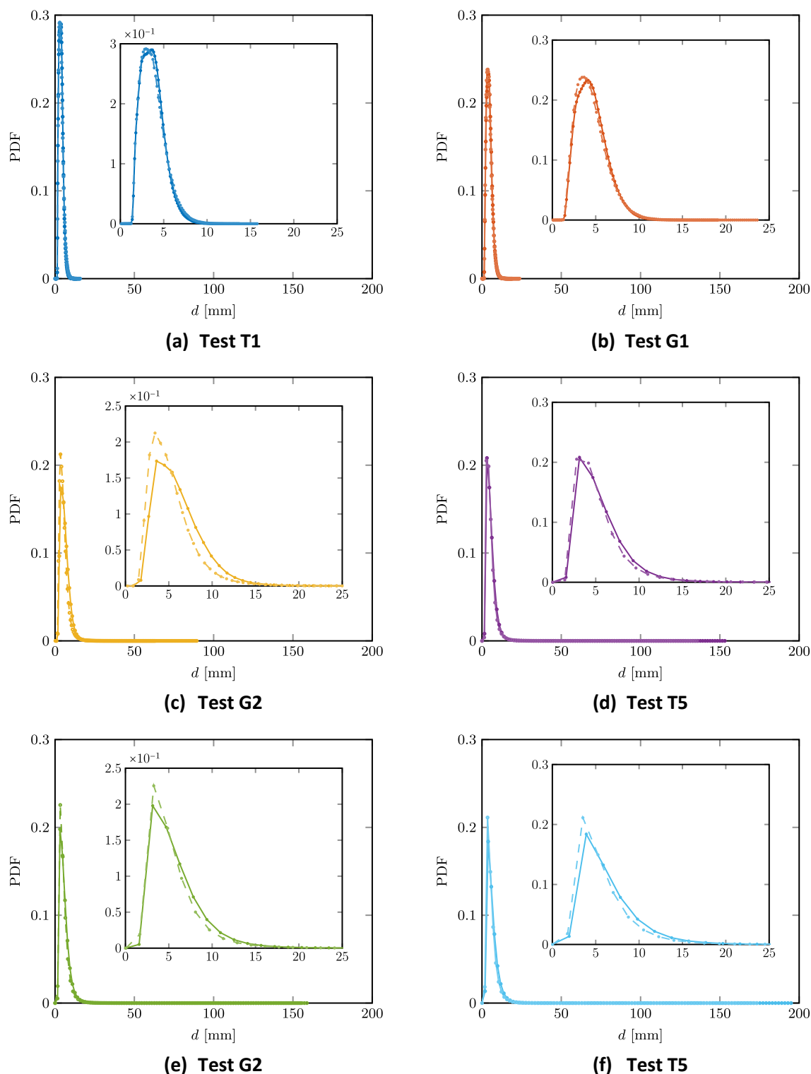
Figure 19: Probability density functions (PDF) representing bubble diameter for different tests for a time interval between 360 and 420 seconds. The solid line corresponds to the upstream, while the dashed line corresponds to the downstream.
